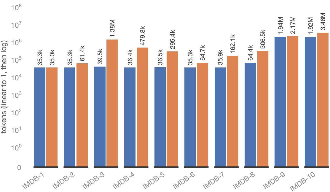
Recomputed KV tokens
