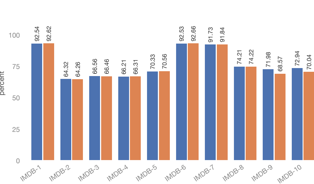
Answer agreement with reference labels
