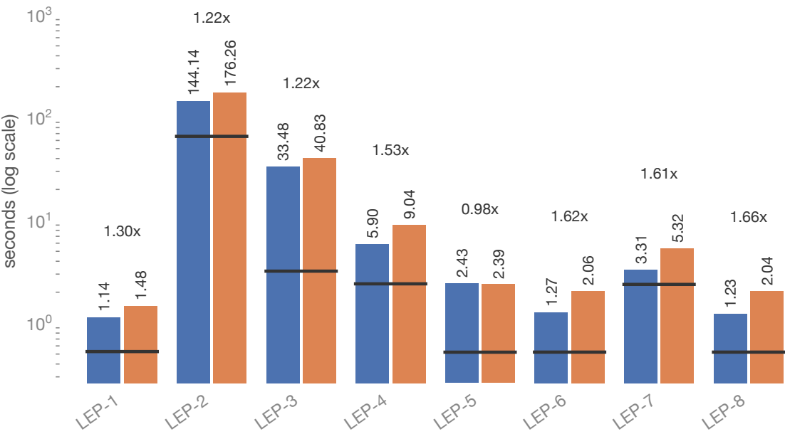
Latency (ratios: vLLM / Quail)
