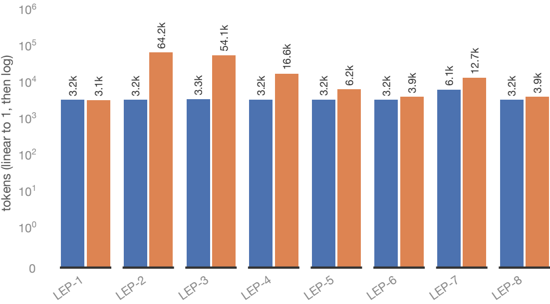
Recomputed KV tokens
