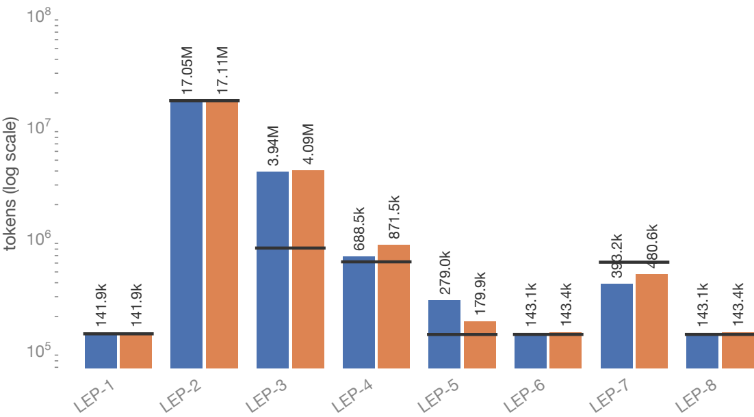
Fresh input tokens
