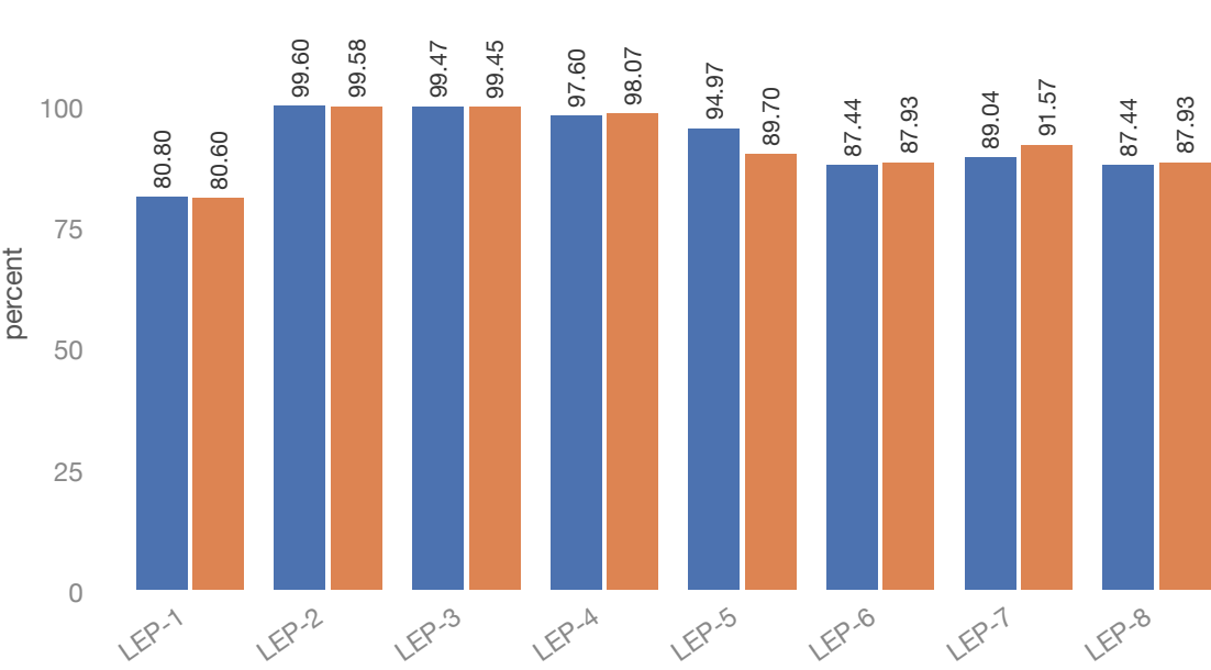
Answer agreement with reference labels
