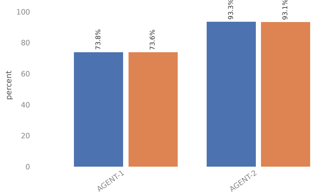
Answer agreement
