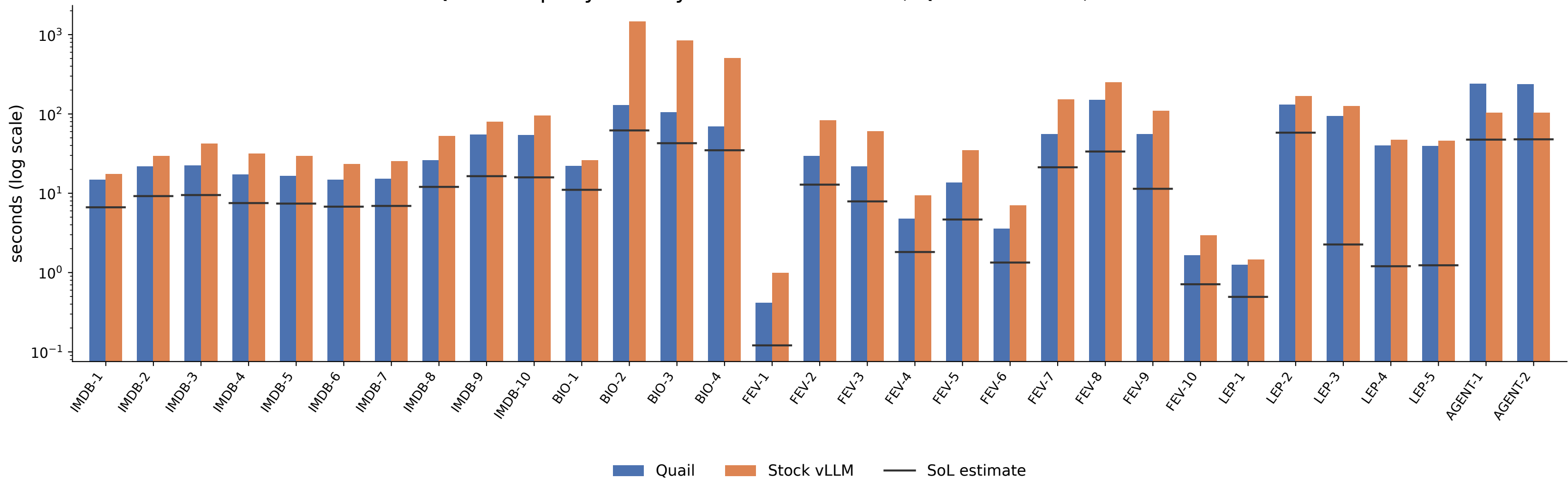
QUAIL-B query latency at scale factor 0.1, Qwen3 4B FP8, one H100
