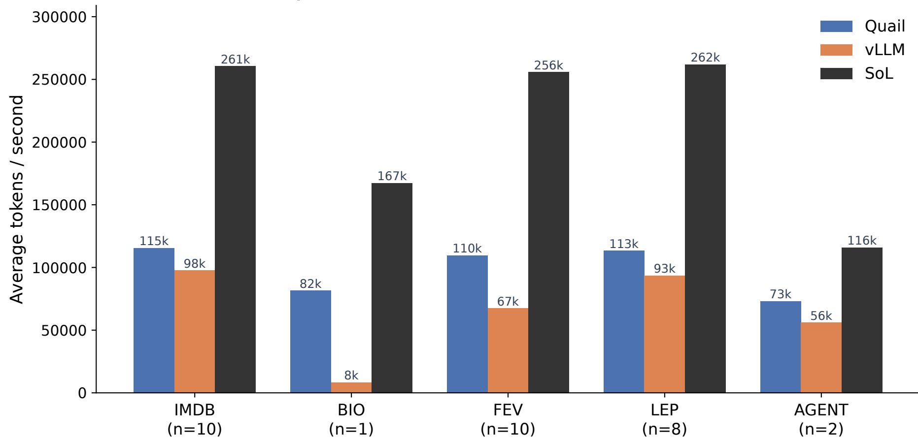
QUAIL-B average tok/sec by dataset Qwen3 4B FP8, one H100, scale factor 0.1
