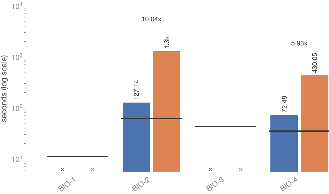
Latency (ratios: vLLM / Quail)
