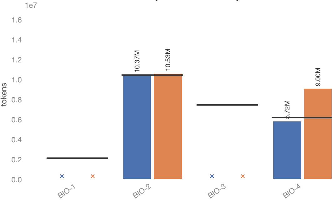
Fresh input tokens computed
