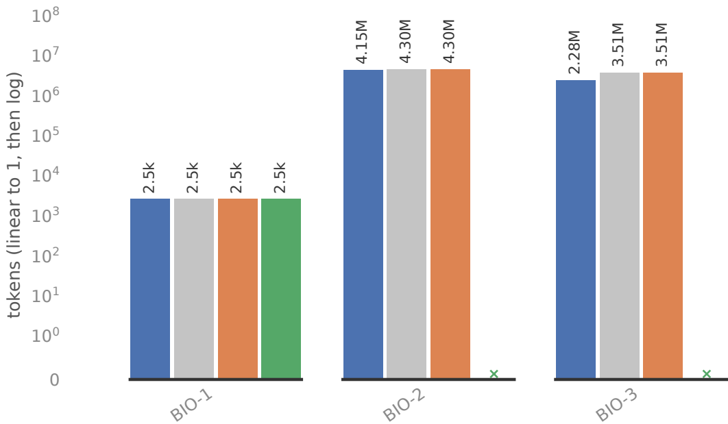
Recomputed KV tokens
