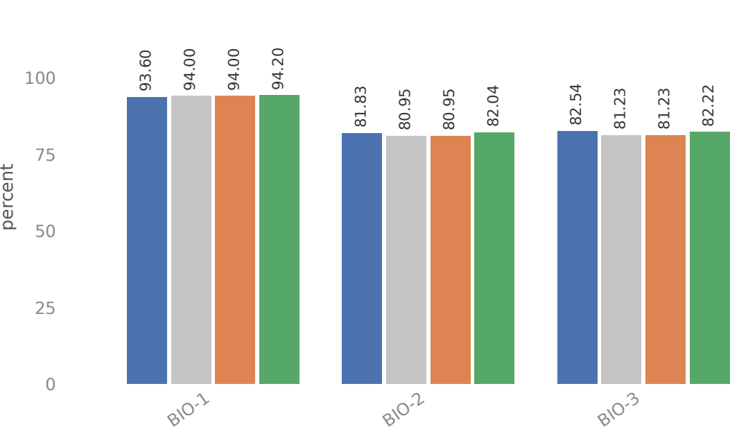
Answer agreement with Qwen3 32B
