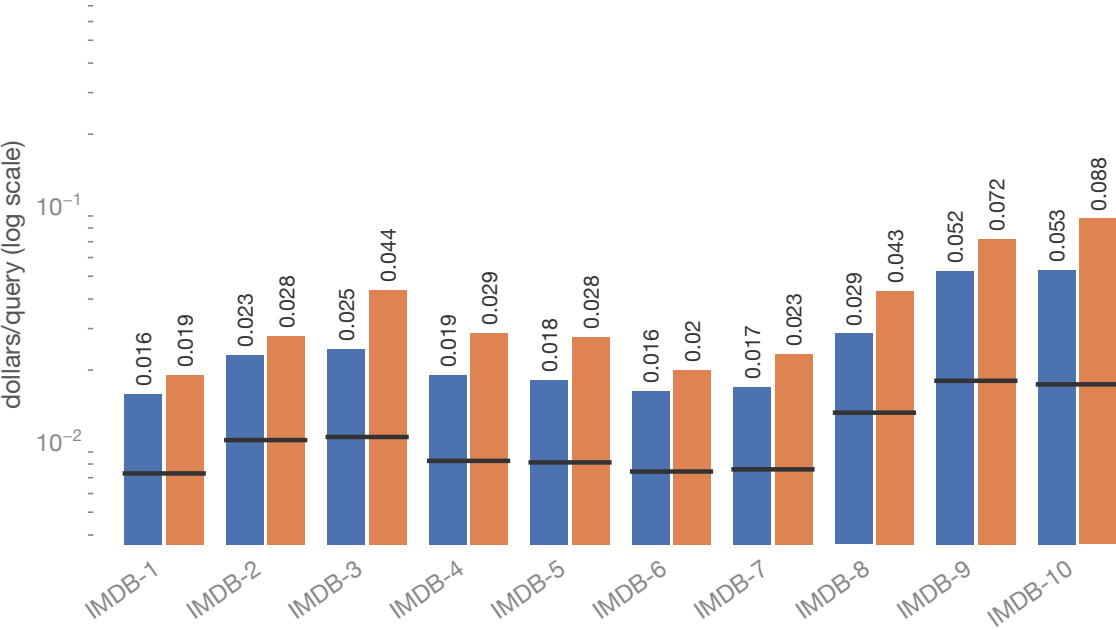
GPU cost per query
