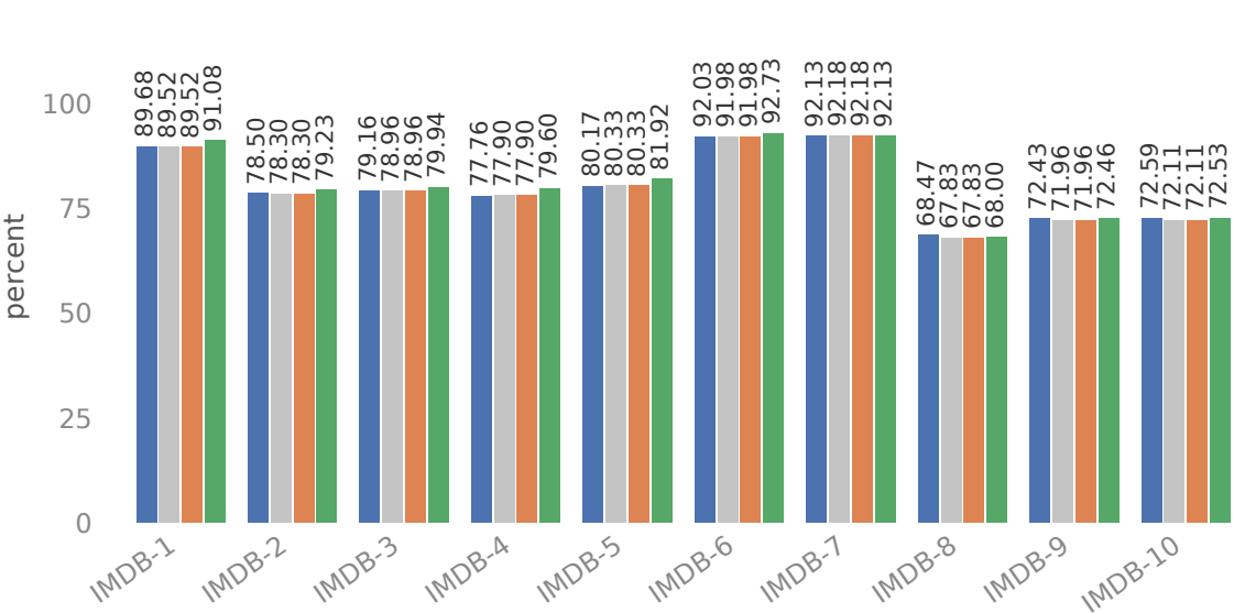
Answer agreement with Qwen3 32B
