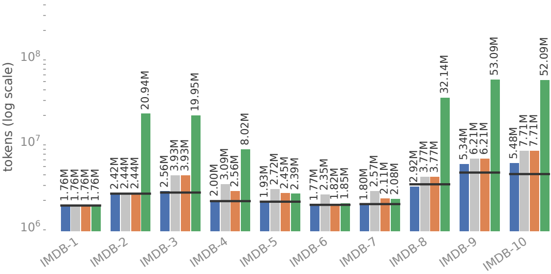
Fresh input tokens
