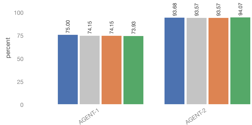
Answer agreement with Qwen3 32B
