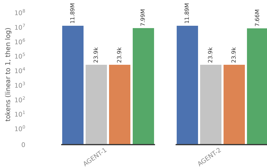
Recomputed KV tokens
