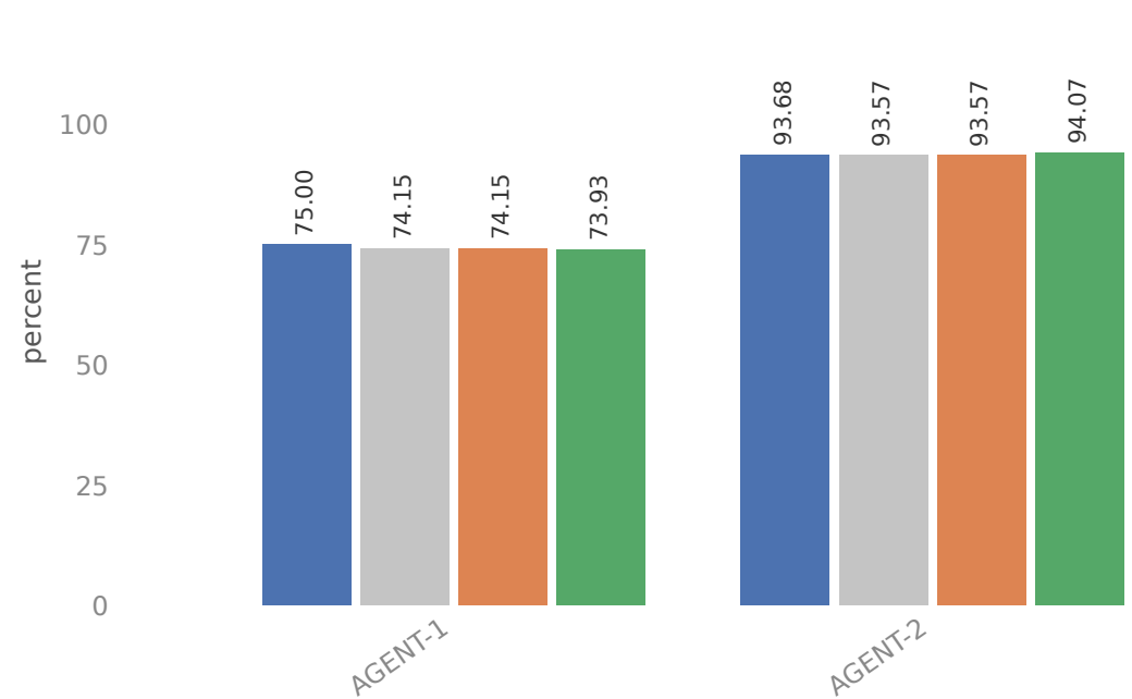
Answer agreement with Qwen3 32B
