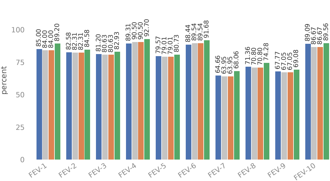
Answer agreement with Qwen3 32B
