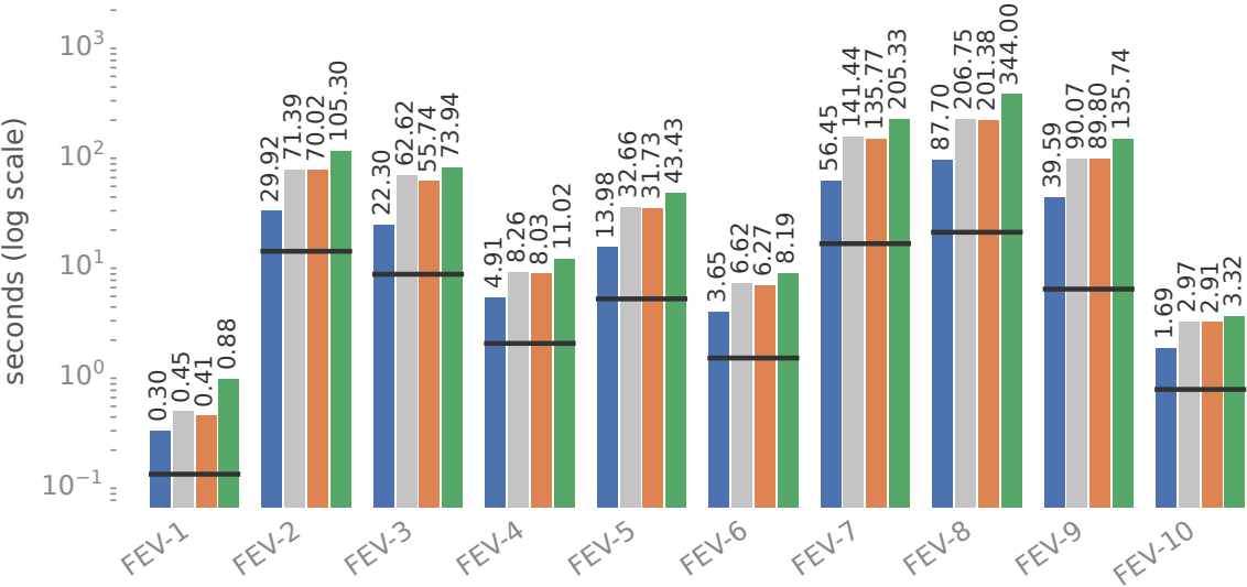
Latency
