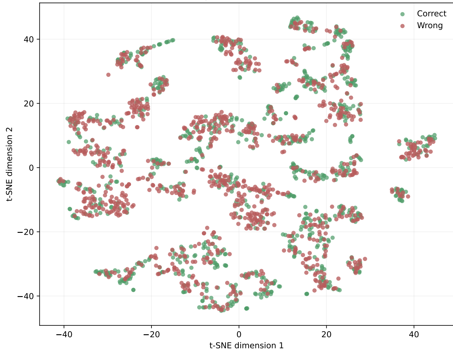
t-SNE Correct vs Wrong (test, n=1987, classifier acc=47.31%)
