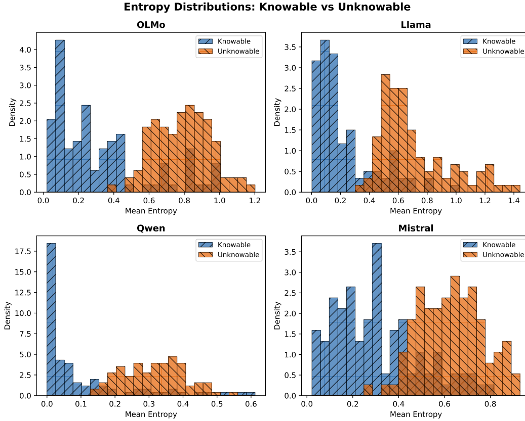
Figure 3: Per-token entropy distributions for knowable vs. unknowable queries. The distributions separate consistently across architectures, with responses to unknowable queries showing higher entropy (mean 0.61 nats) than responses to knowable ones (0.24).
