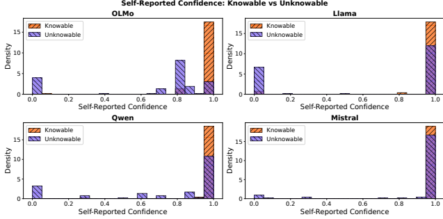
Figure 1. All four models report high confidence on unknowable queries
