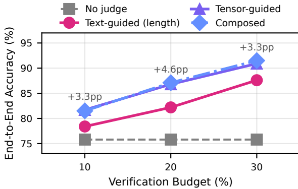
Figure 3. End-to-end accuracy vs. verification budget for four judge conditions, with the 800 responses from four architectures pooled under one budget.
