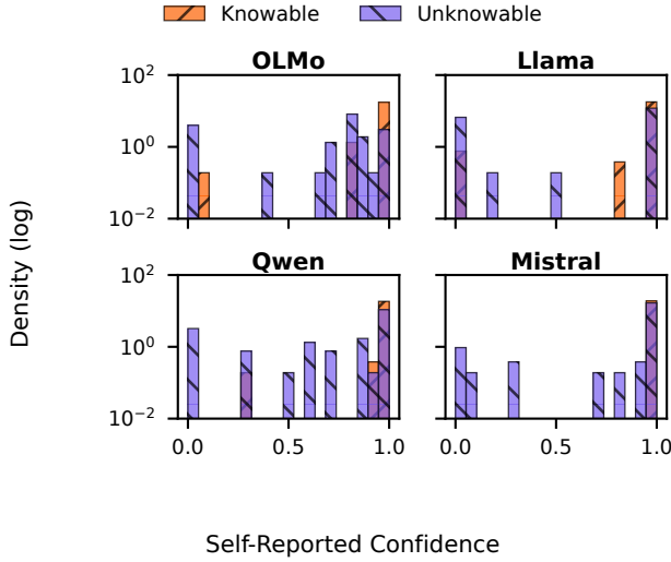
Figure 1. Model confidence on unknowable queries
