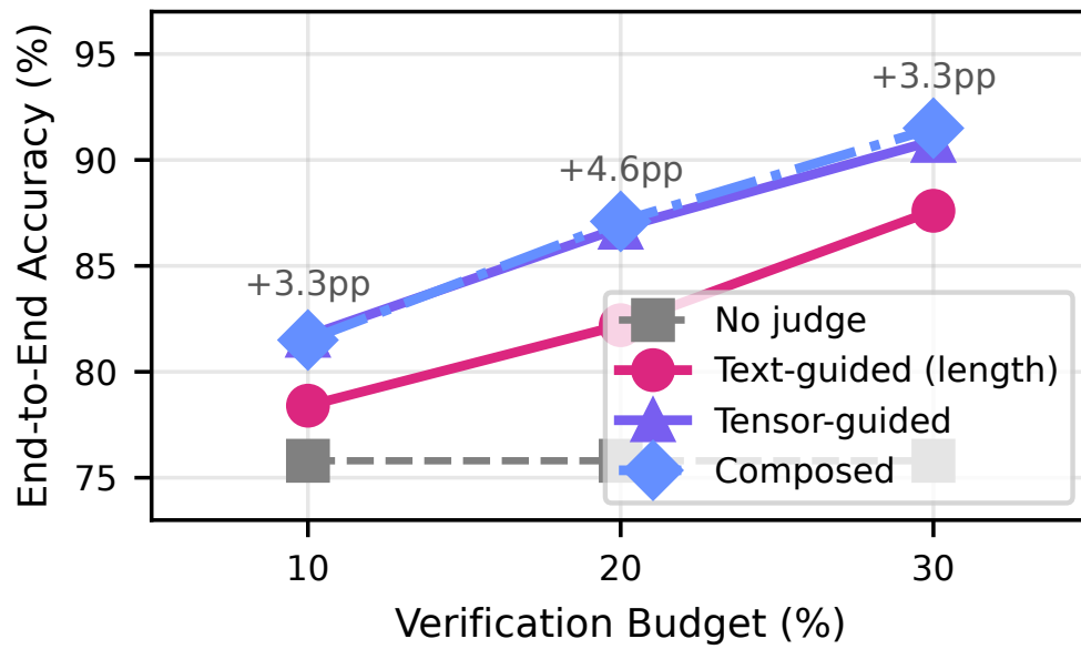
Figure 2: Aggregate budget curve across all models: accuracy as a function of verification budget for each judge strategy. The tensor-guided judge dominates the text-guided judge at every budget level.
