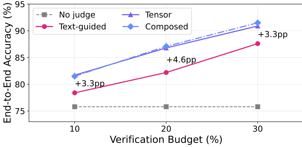
Figure 2: Aggregate budget curve across all models: accuracy as a function of verification budget for each judge strategy. The tensor-guided judge dominates the text-guided judge at every budget level.
