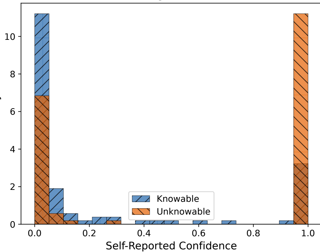
Qwen
