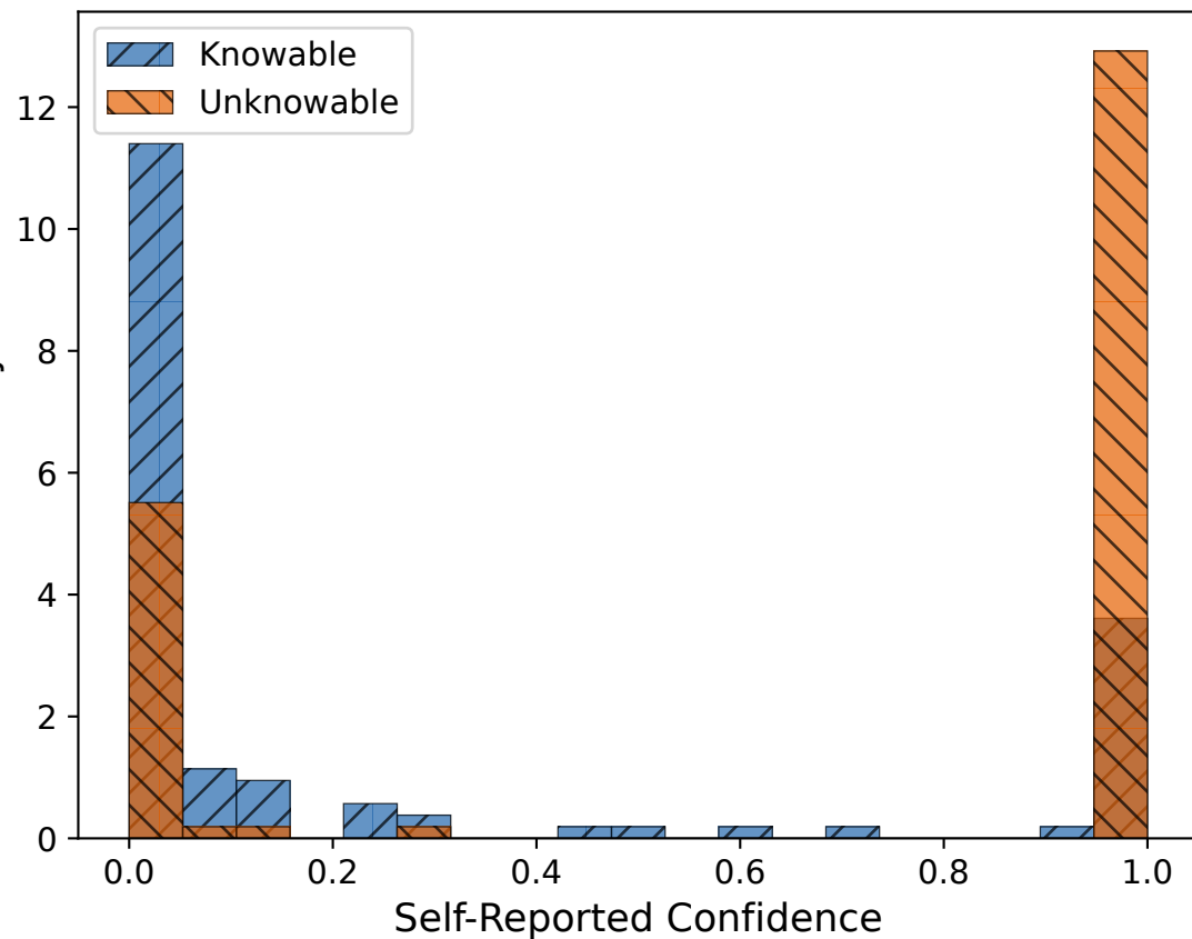
Qwen
