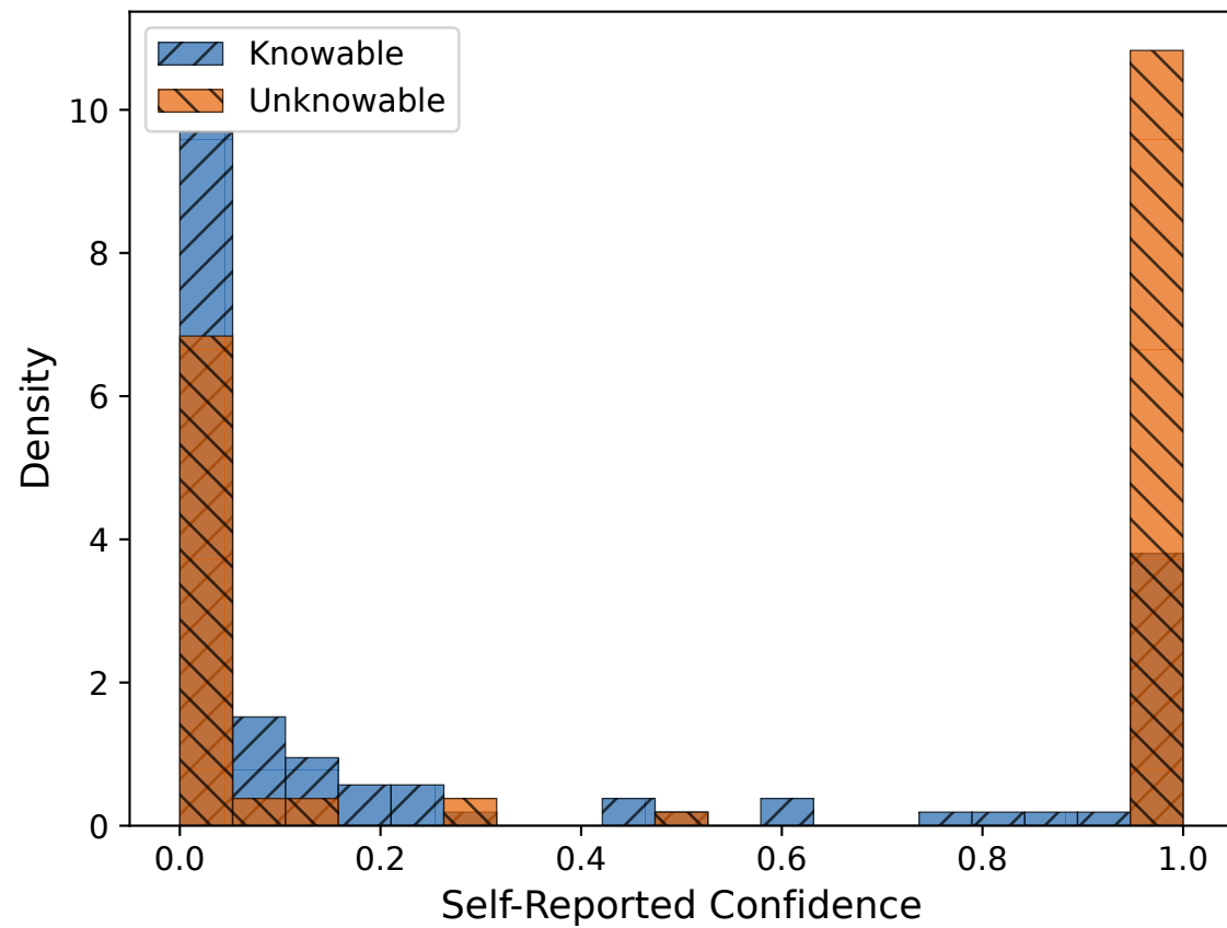
Mistral
