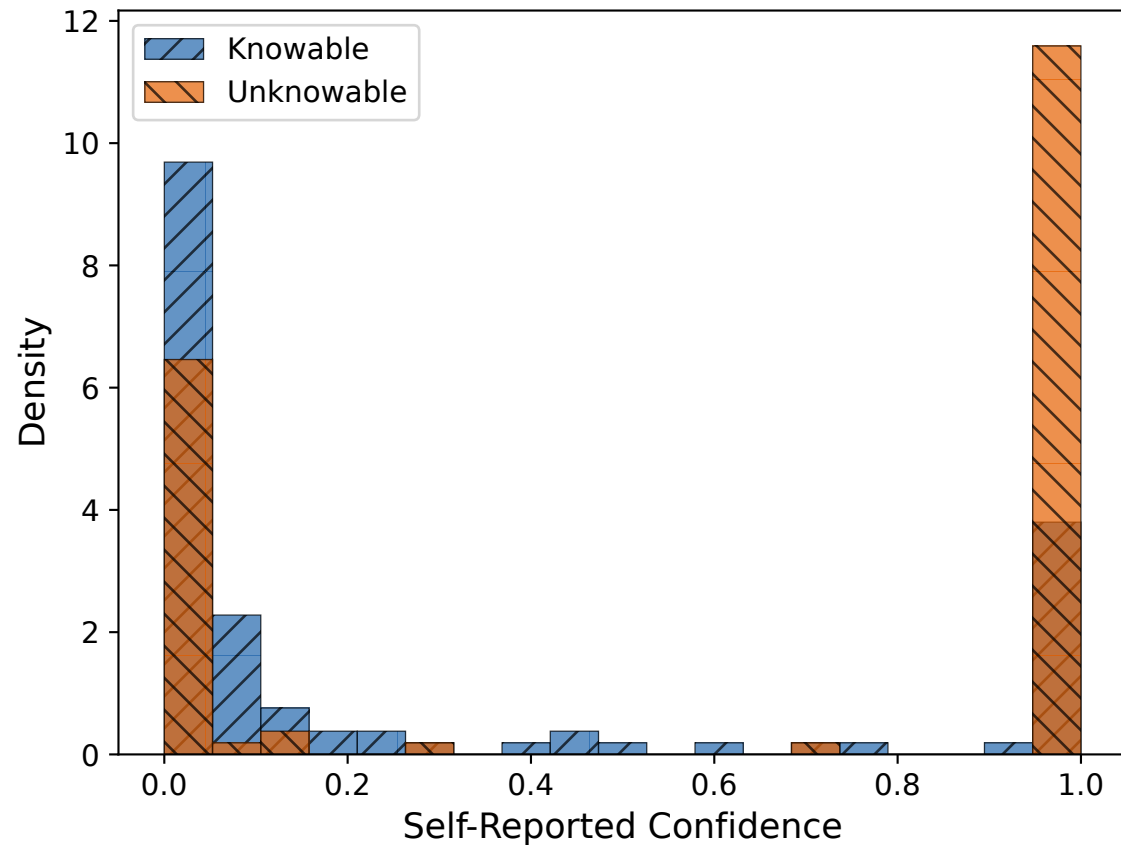
Mistral
