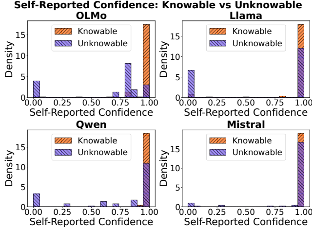
Figure 1. All four models report high confidence on unknowable queries
