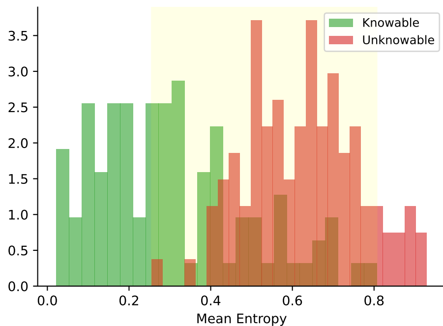
Mistral
