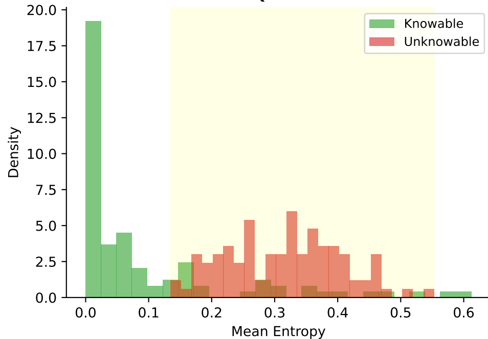
Qwen
