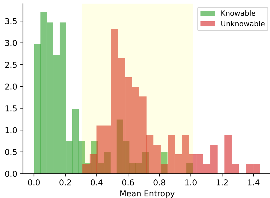
Mistral
