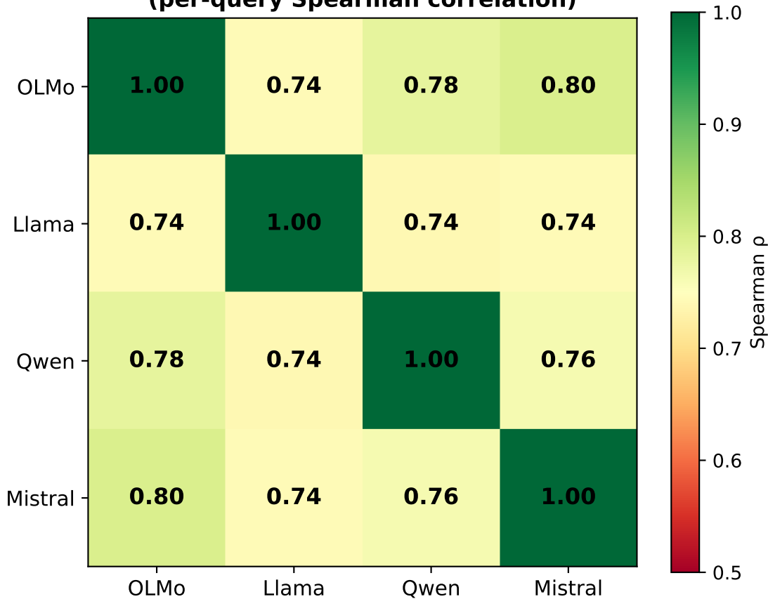
Cross-Model Entropy Agreement (per-query Spearman correlation)
