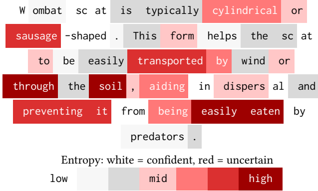
Figure 2. Generated output along with its entropy trace for the query What shape is wombat scat? The generated answer is a fabrication—wombat scat is distinctively cube-shaped. The trace illustrates exported telemetry, not a token-level truth detector.
