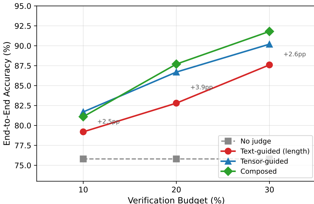
Figure 1: Aggregate budget curve across all models: accuracy as a function of verification budget for each judge strategy. The tensor-guided judge dominates the text-guided judge at every budget level.
