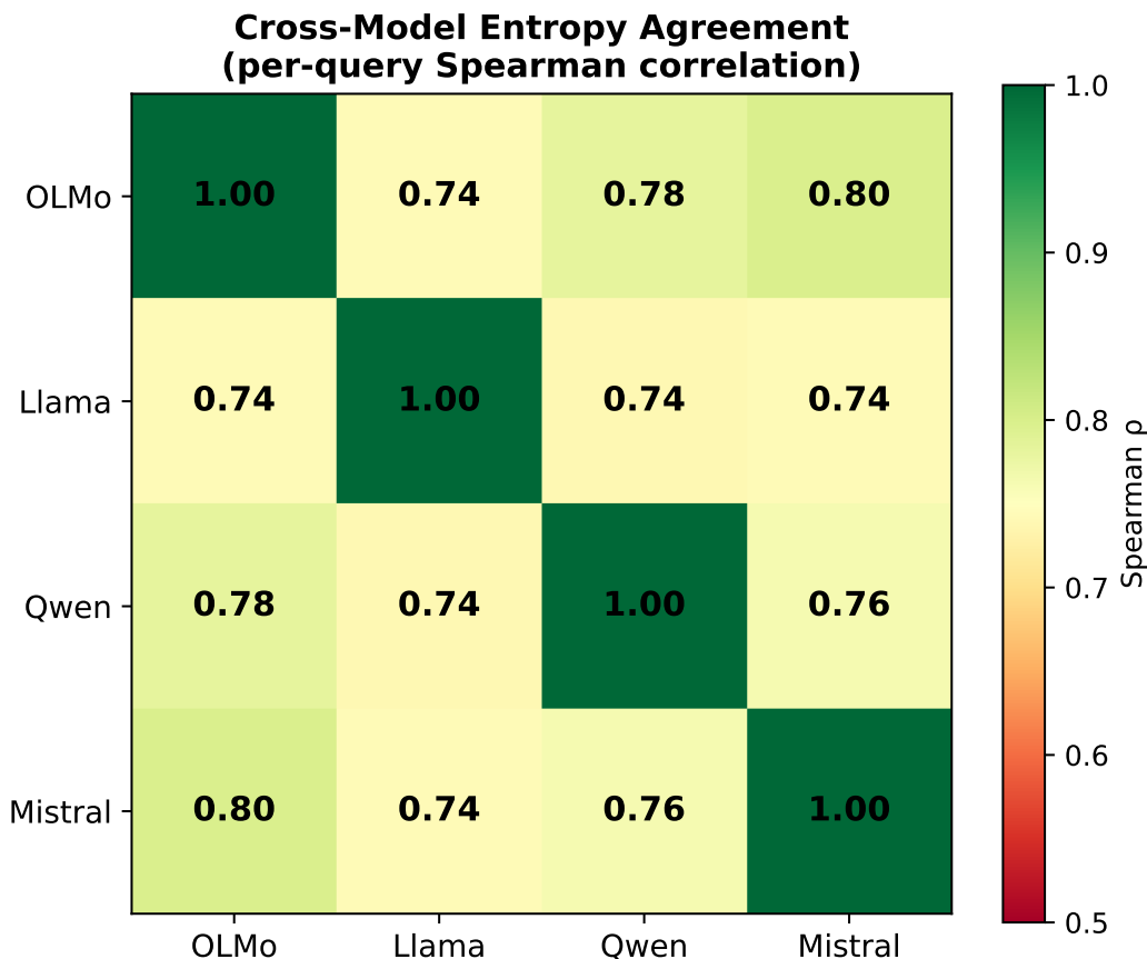
Figure 3: Cross-model entropy correlation. Spearman \rho = 0.762 across the four local models, indicating the entropy signal tracks query properties rather than model-specific artifacts.
