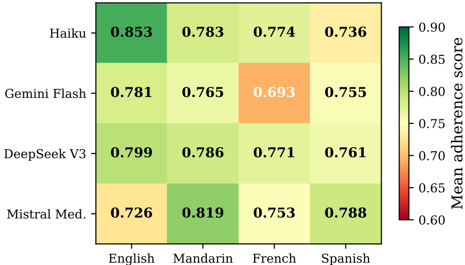
Mean Instruction Adherence by Model and Language
