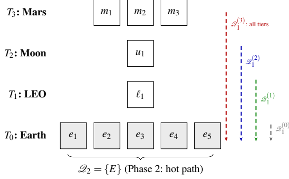
Figure 3: The crumbling-wall construction over the 5/1/1/3 topology. Each tier's Phase 1 quorum reads downward through the wall (dashed arrows). Phase 2 uses only the Earth row (shaded). The wall narrows from bottom to top: wider rows offer more quorum choices.
