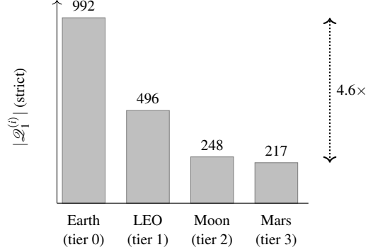
Figure 2: Phase 1 quorum count by initiating tier under the strict wall. The values are exhaustive structural counts over the fixed 5/1/1/3 configuration; no connectivity distribution, timeout, or stochastic trial is assumed.
