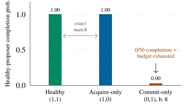
Figure 2: Pre-registered single-decree contention experiment (50 seeds per cell). The prediction that an acquire-only (1, 0) incumbent would be more disruptive was reversed: it matched the healthy baseline on every recorded metric, while a commit-only (0, 1) incumbent with a round budget of 8, which is equal to the healthy proposer’s own fixed budget, exhausted the healthy proposer’s progress budget (0/50 completions, drawn as a minimal stub for visibility).
