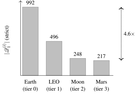
Figure 4: Phase 1 quorum count by initiating tier under the strict wall. The values are exhaustive structural counts over the fixed 5/1/1/3 configuration; no connectivity distribution, timeout, or stochastic trial is assumed.
