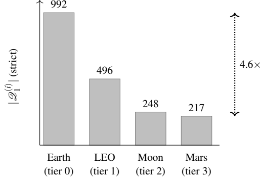
Figure 2: Phase 1 quorum count by initiating tier under the strict wall. The values are exhaustive structural counts over the fixed 5/1/1/3 configuration; no connectivity distribution, timeout, or stochastic trial is assumed.
