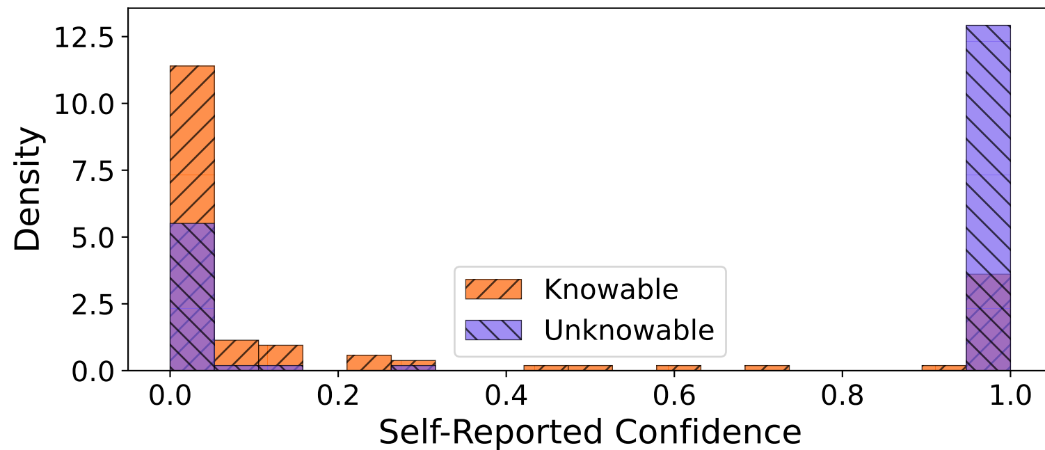
Qwen
