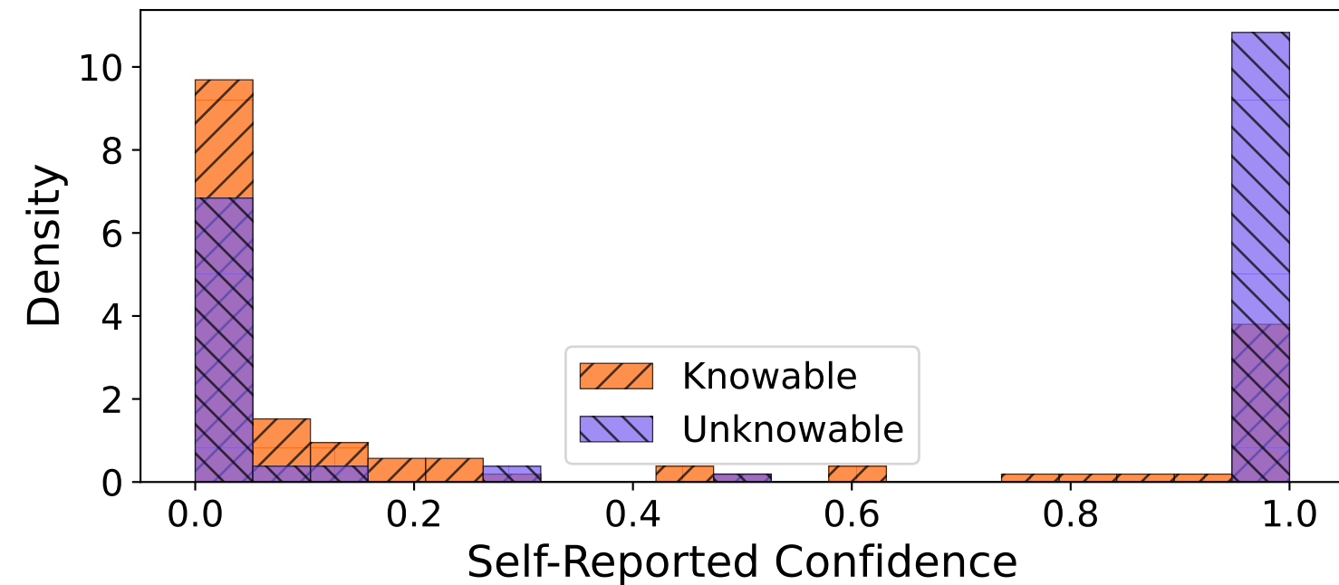
Mistral
