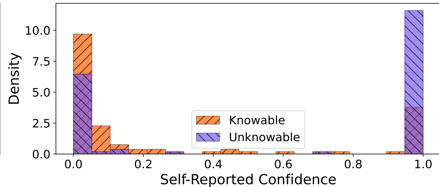
Mistral
