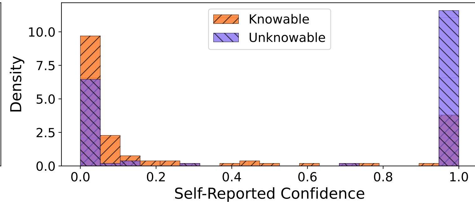
Mistral
