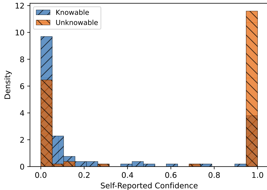
Mistral
