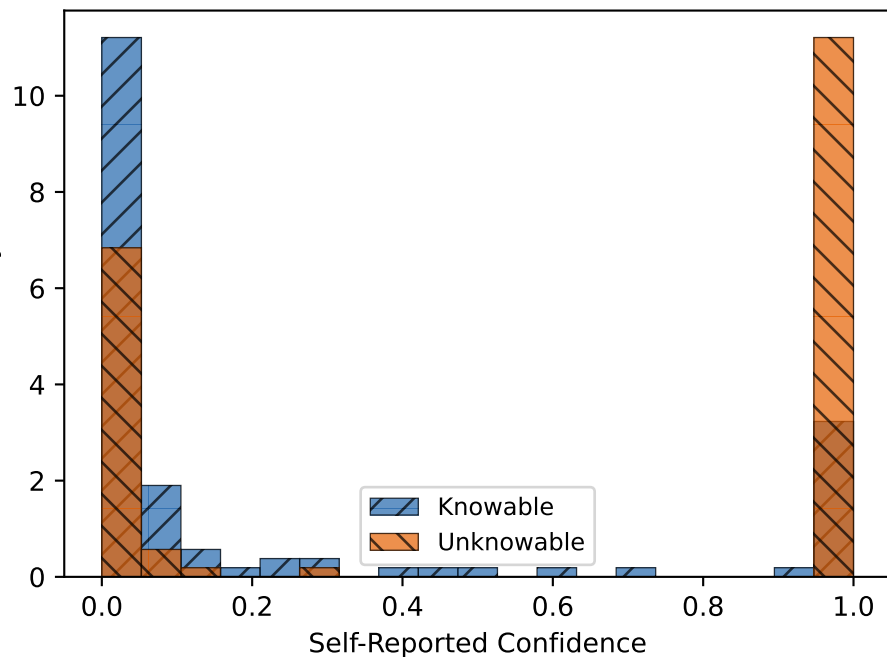
Qwen
