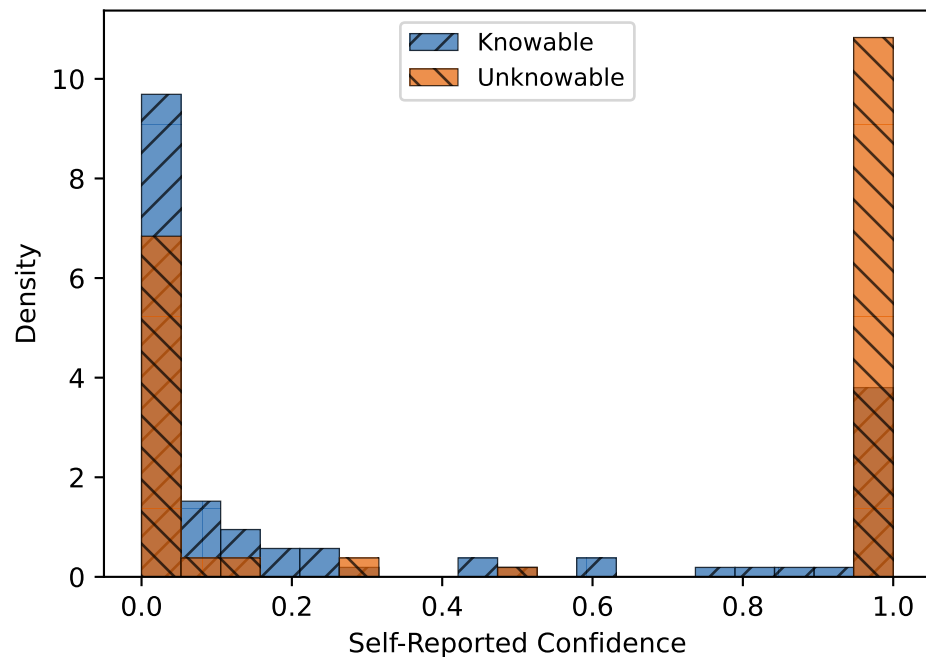
Mistral
