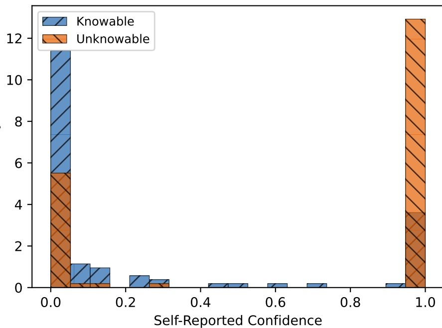
Qwen
