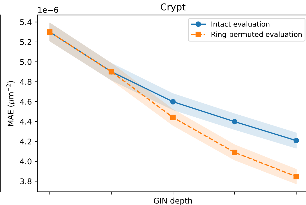
Intact-trained GIN: intact vs ring-permuted evaluation Mean \pm SEM across validation organoids
