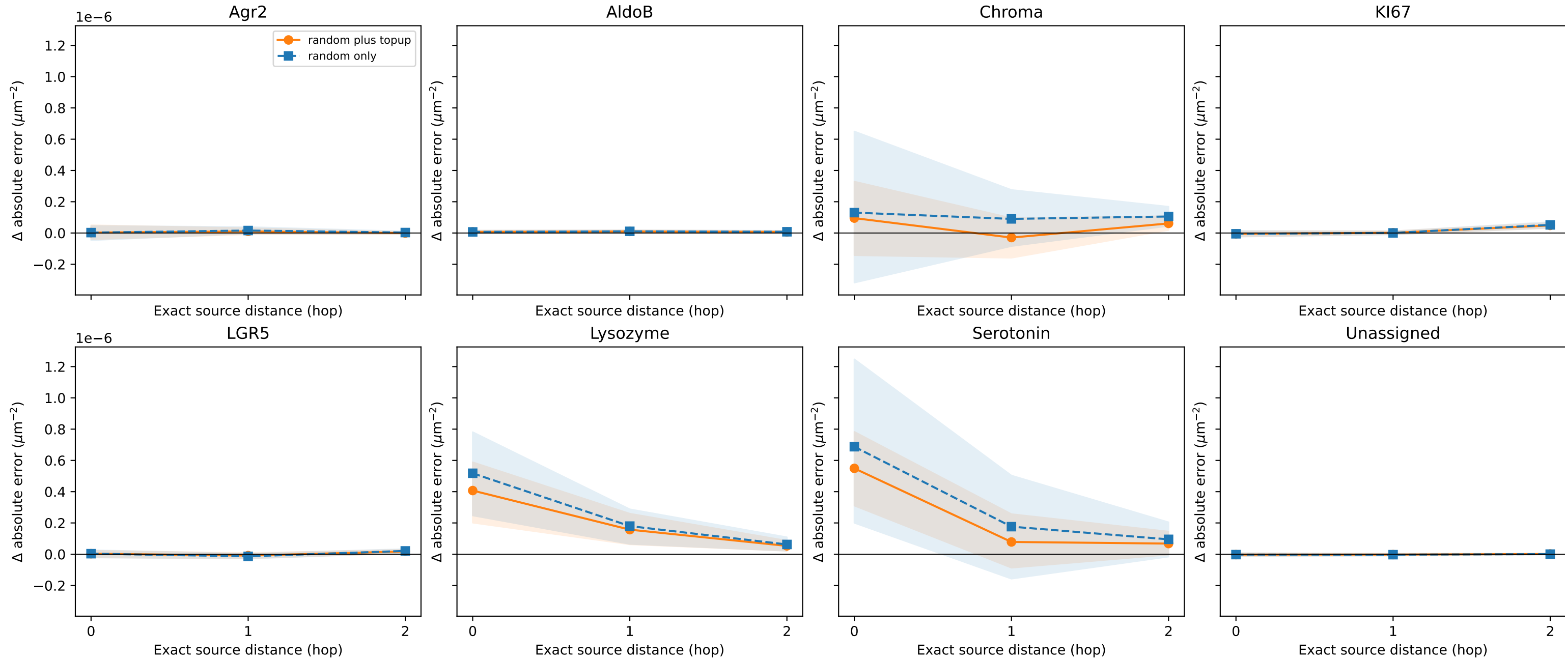
One masked source; all recipient lineages pooled; organoid-bootstrap 95% intervals
