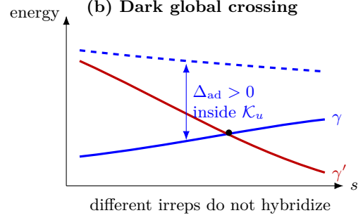
Figure 1: Protocol-dependent spectral relevance. (a) The joint-fixed space is only symmetry allowed; the cyclic space also depends on the initial state and generated algebra. (b) A branch in another irrep can cross the followed branch and close a global multiplicity gap while the tracked band remains isolated within the cyclic space.
