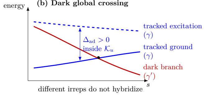
Figure 1: Protocol-dependent spectral relevance. (a) The joint-fixed space is fixed by symmetry; the cyclic envelope also depends on the initial state and generated algebra, while a specified schedule traces \mathcal{R}_u[s(\cdot)] inside it. Membership in \mathcal{K}_u alone does not imply state reachability. (b) The labels \gamma and \gamma' denote inequivalent symmetry sectors. A branch in the latter can cross the followed branch and close a global multiplicity gap while the tracked band remains isolated within the cyclic envelope. Solid blue is the tracked ground branch, dashed blue its in-sector excitation, and red an inequivalent dark branch. Panel (b) depicts the transverse mechanism of Theorem 7, not the simultaneous diagonal cancellation of Theorem 6; the diagram is not to scale.
