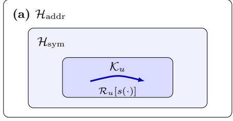
symmetry fixes \mathcal{H}_{\text{sym}} ; the generators select \mathcal{K}_u
