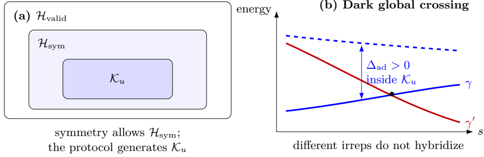
Figure 1: Protocol-dependent spectral relevance. (a) The joint-fixed space is only symmetry allowed; the cyclic space also depends on the initial state and generated algebra. (b) A branch in another irrep can cross the followed branch and close a global multiplicity gap while the tracked band remains isolated within the cyclic space.
