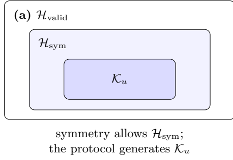
Figure 1: Protocol-dependent spectral relevance. (a) The joint-fixed space is only symmetry allowed; the cyclic space also depends on the initial state and generated algebra. (b) A branch in another irrep can cross the followed branch and close a global multiplicity gap while the tracked band remains isolated within the cyclic space.
