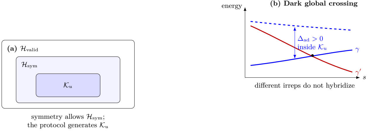
Figure 1: Protocol-dependent spectral relevance. (a) The joint-fixed space is only symmetry allowed; the cyclic space also depends on the initial state and generated algebra. (b) A branch in another irrep can cross the followed branch and close a global multiplicity gap while the tracked band remains isolated within the cyclic space.
