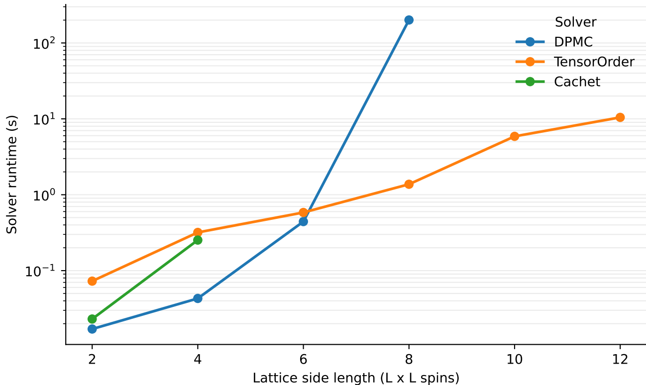
2D Ising model runtime
