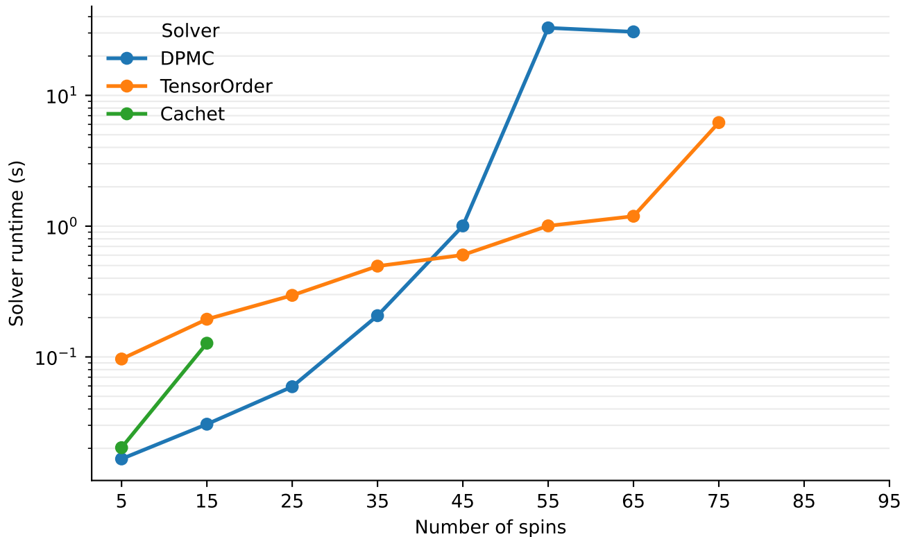
Random graph Ising model runtime
