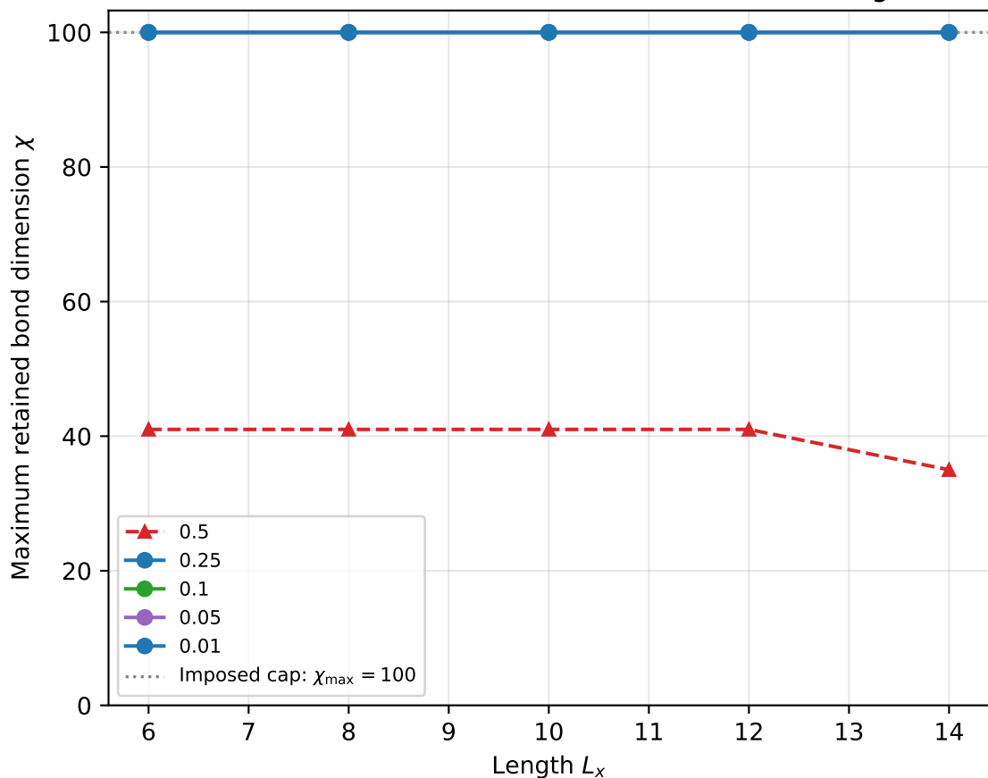
Maximum Bond Dimension: Random Bond Ising
