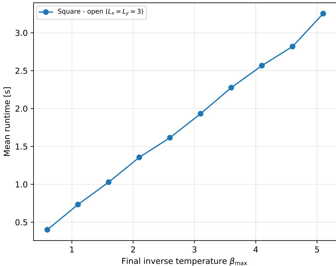
Runtime versus inverse temperature: Random Bond Ising
