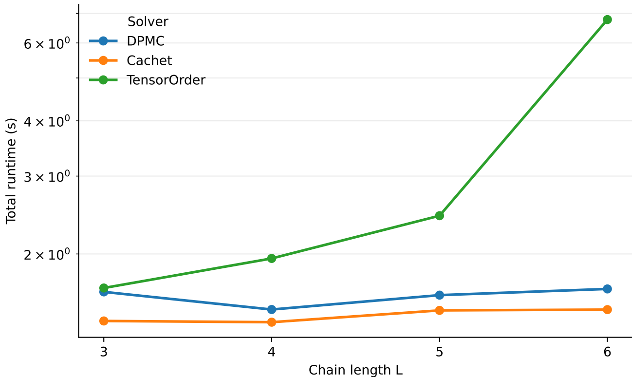
1D Ising model runtime
