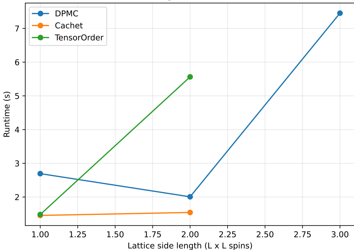
2D Ising model runtime
