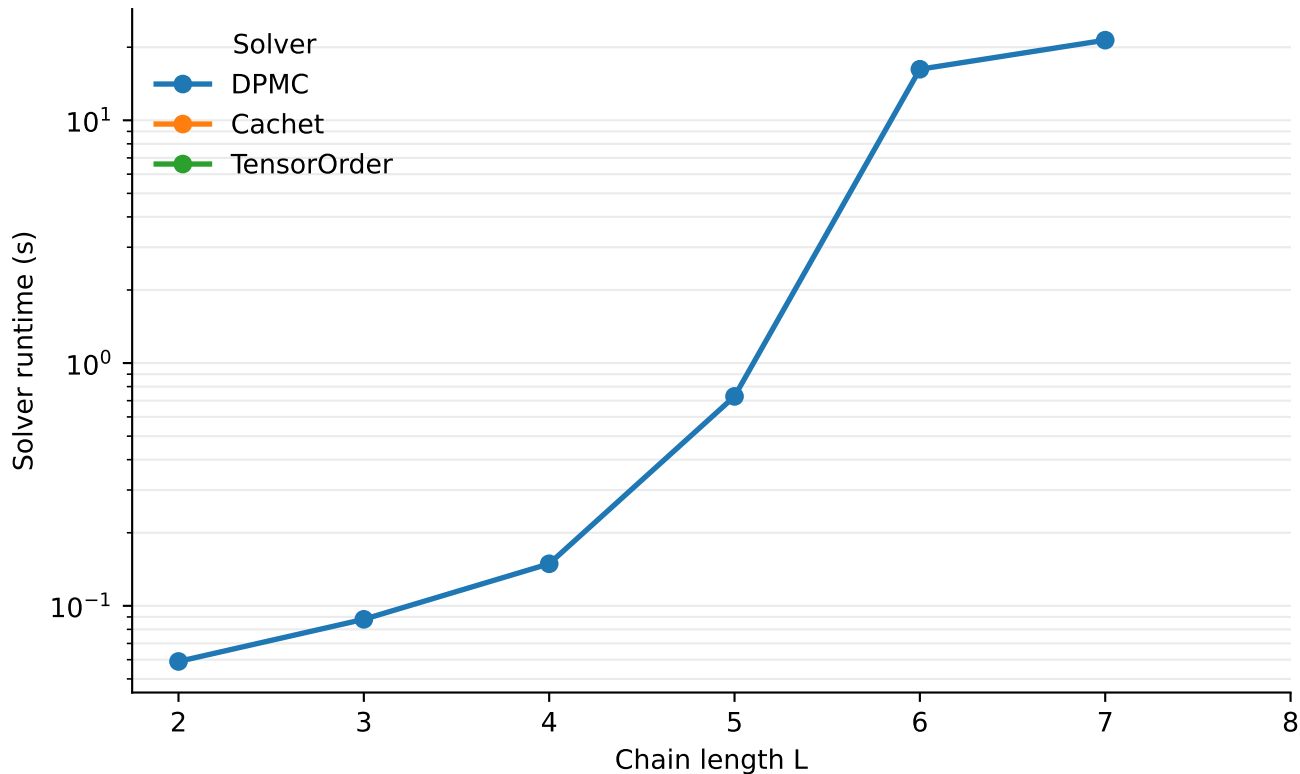
Transverse-field Ising runtime (10 Trotter steps)
