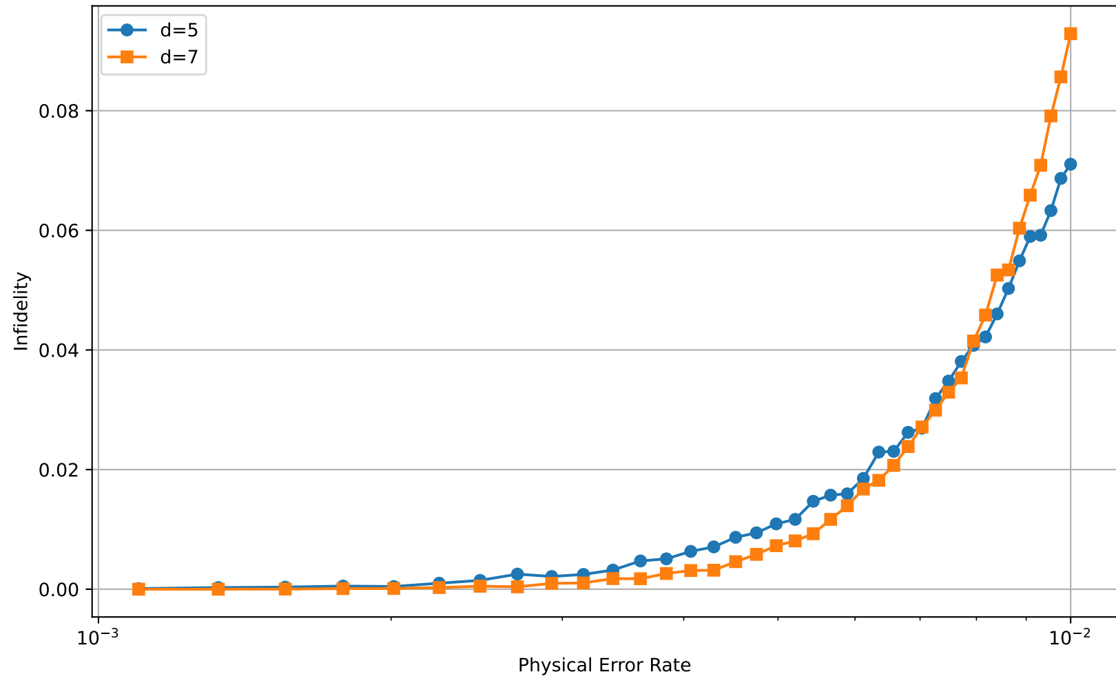
Infidelity vs Physical Error Rate
