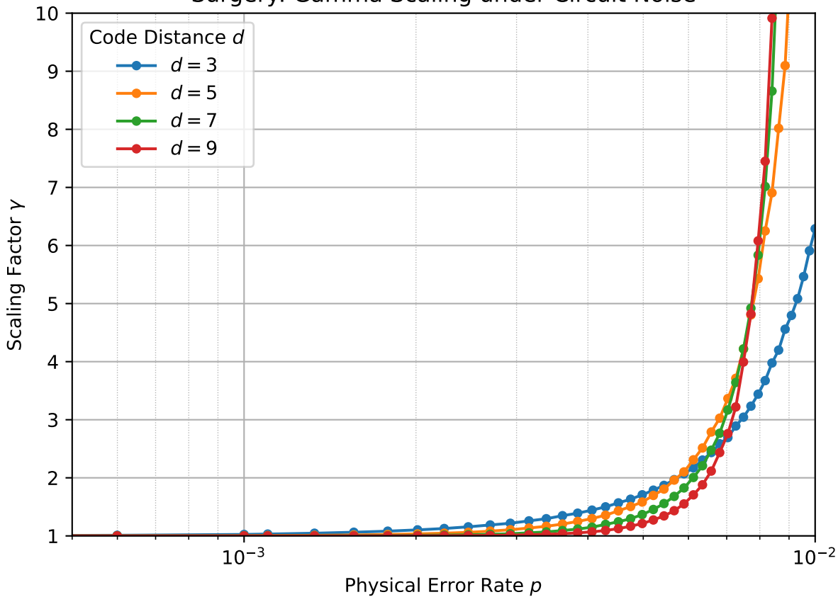
Surgery: Gamma Scaling under Circuit Noise
